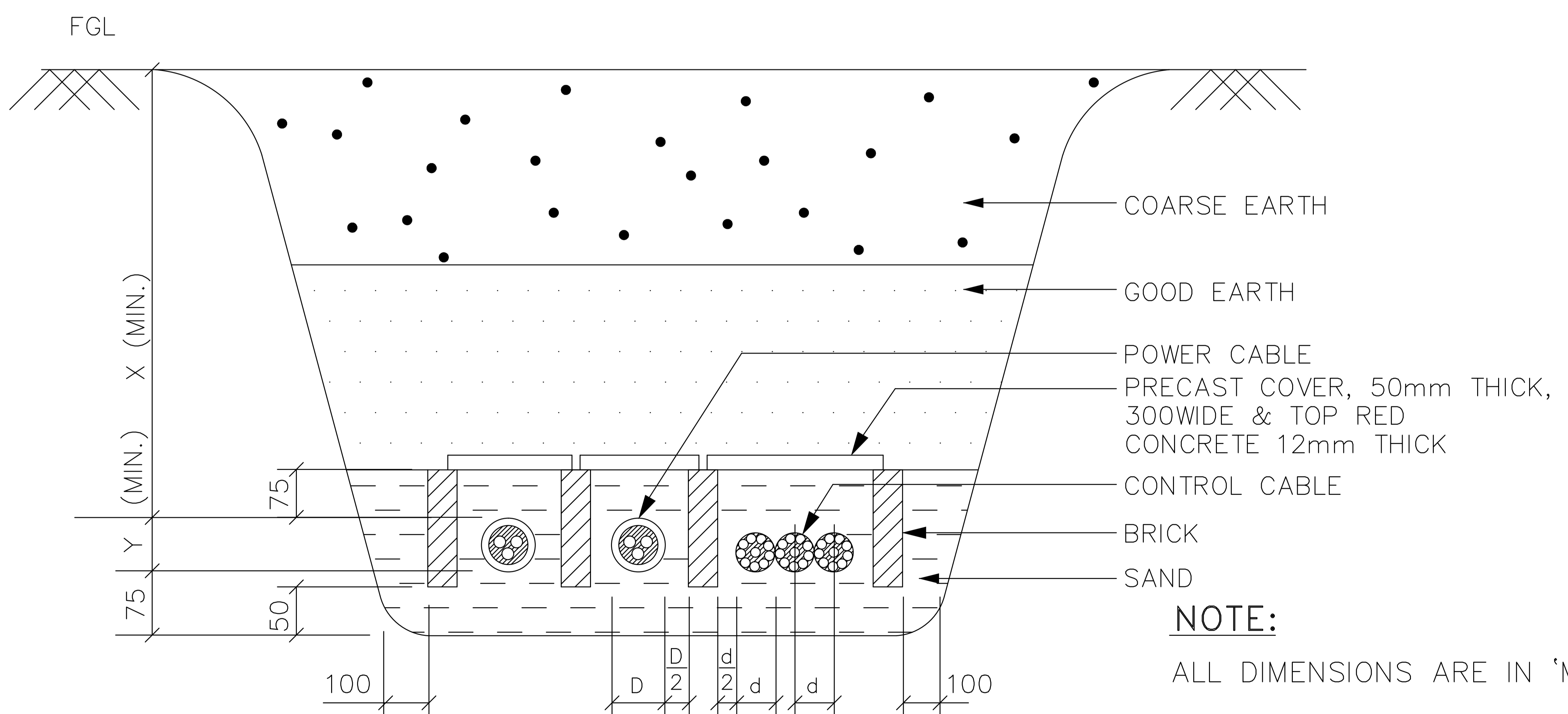
BURIED CABLE LAYING DETAILS
