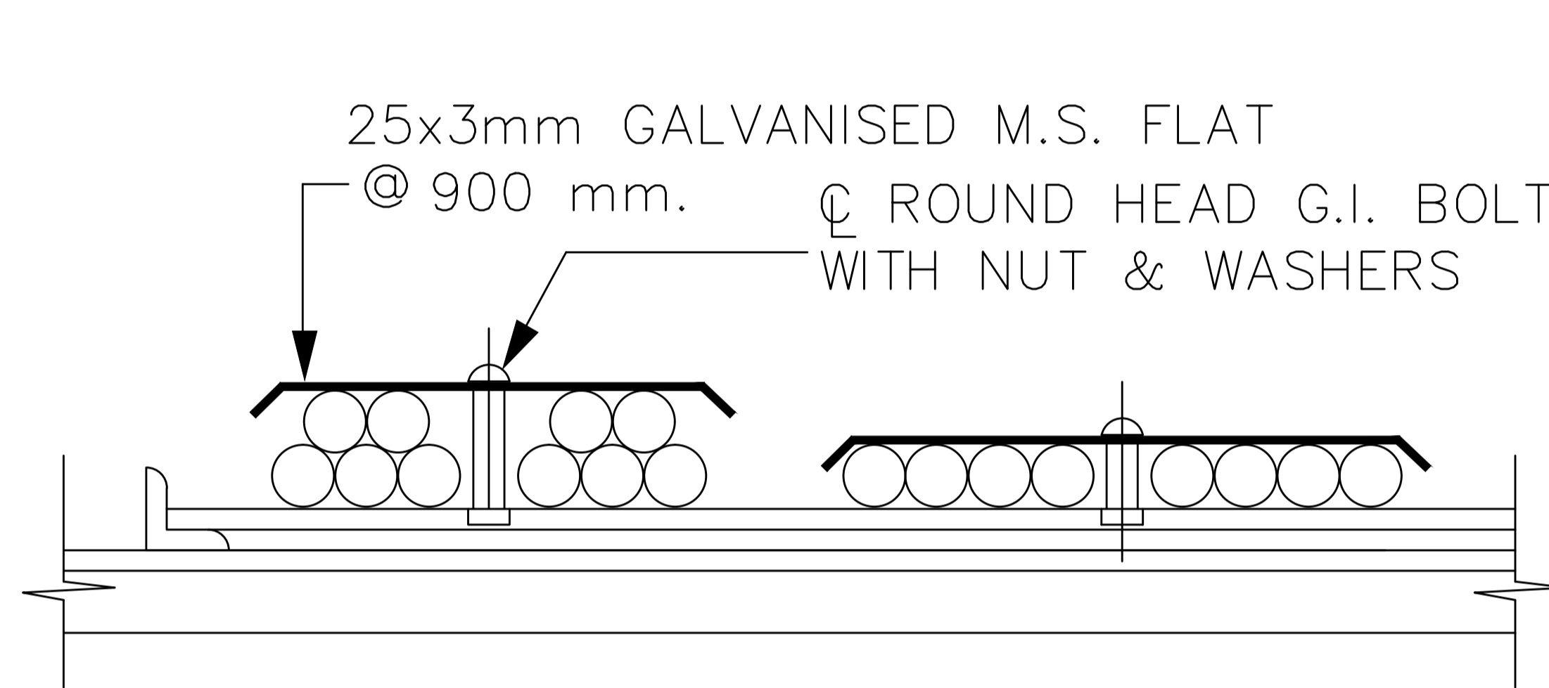
CLAMPING ARRANGEMENT OF CONTROL CABLES
